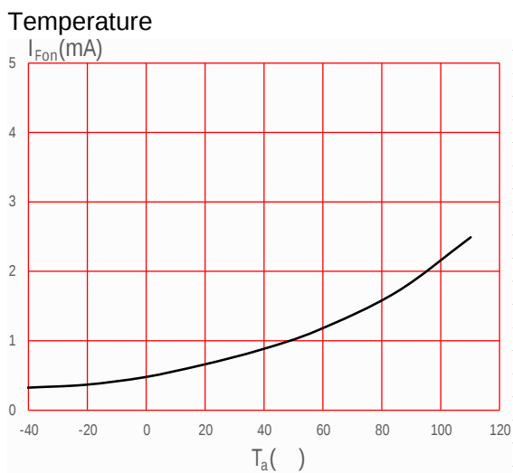
LED Operate Current vs. Ambient
