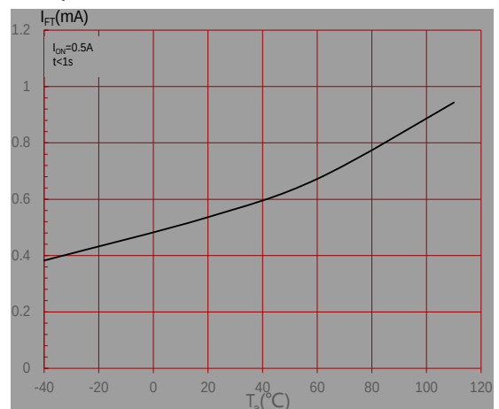
Trigger LED Current vs. Ambient Temperature
