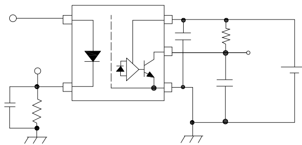
Fig.9: Switching Time Test Circuit and Waveform
