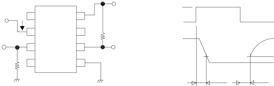
Fig.10: Switching Time Test Circuit and Waveform
