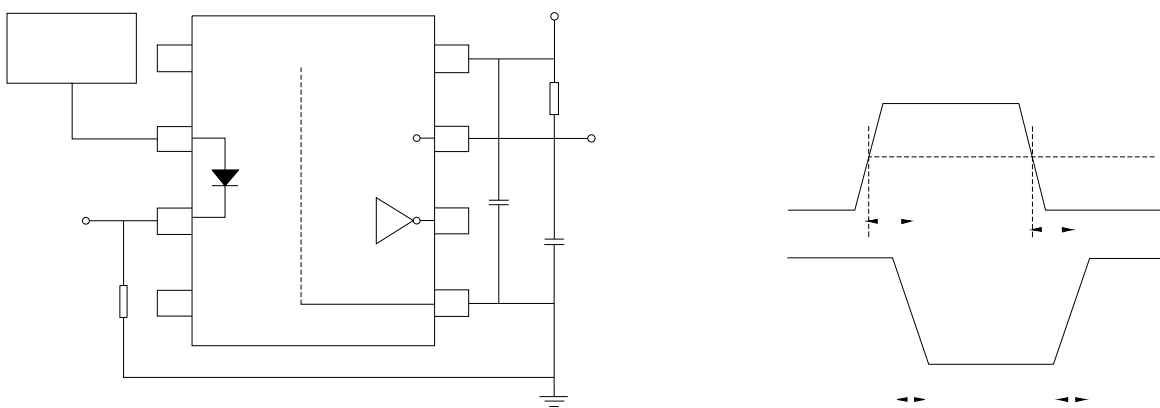
Fig.15: Test Circuit for TPHL and TPLH
