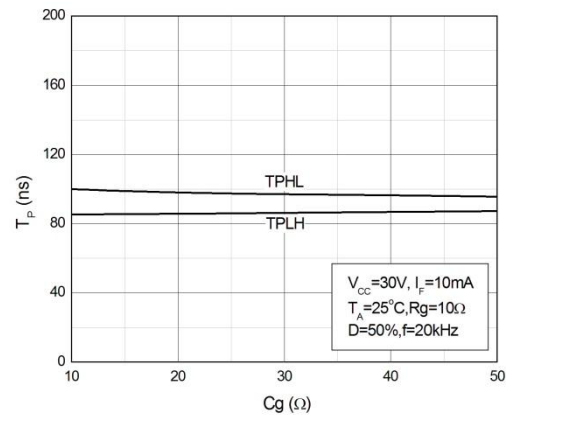
Fig.16 Propagation Delay vs. Load Capacitance
